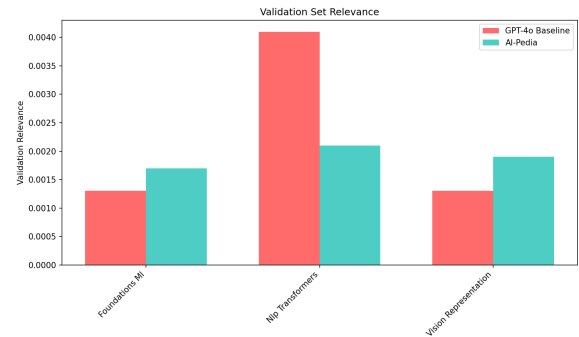
Fig. 10. Validation Set Relevance: Free-form LLM vs AI-Pedia.
