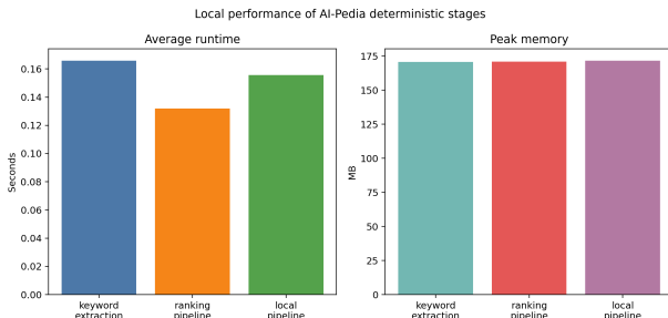
Fig. 8. Runtime and peak memory for deterministic local stages.
