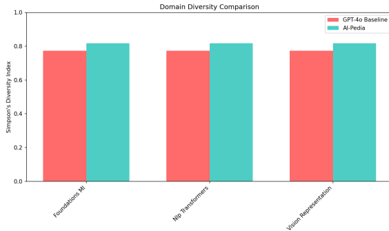
Fig. 9. Domain Diversity: Free-form LLM Baseline vs AI-Pedia Structured Pipeline.
